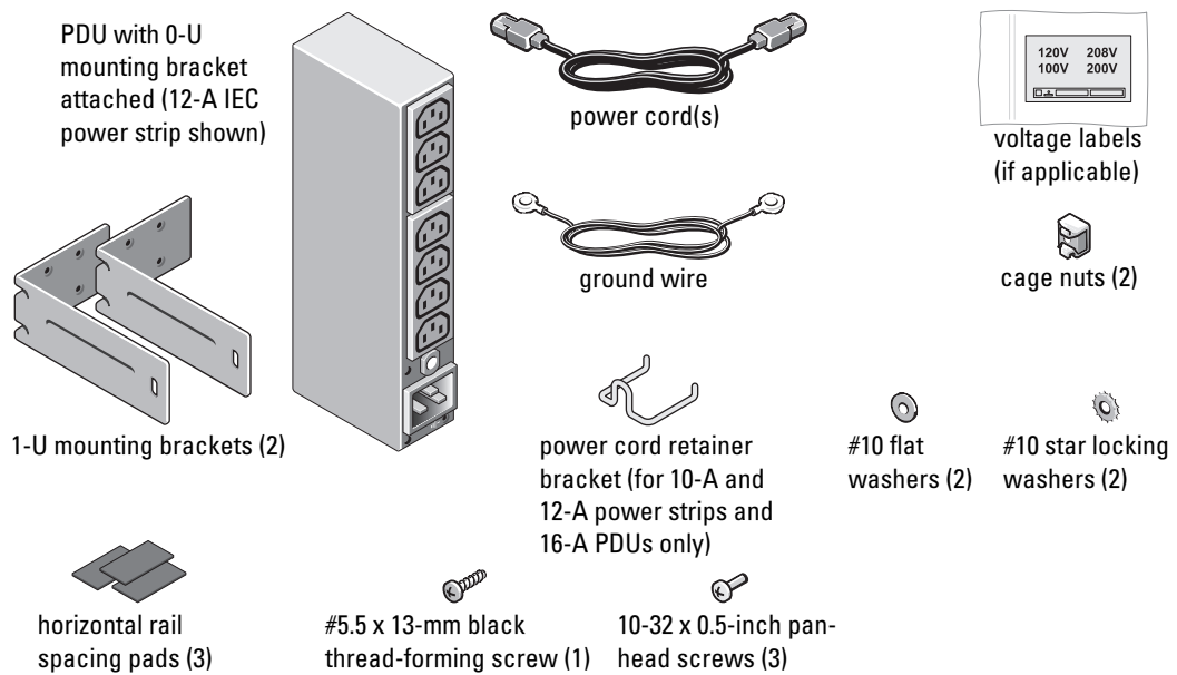
Figure 1-2. Kit Contents
